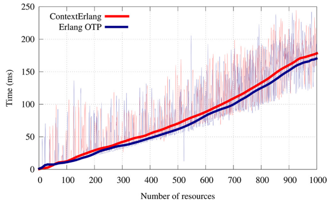
Fig. 17. Performance comparison for the autonomic storage server.
