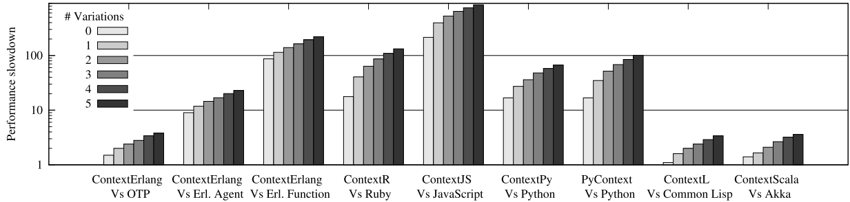
Fig. 16. Performance of layered methods compared to the basic methods in various COP languages.
