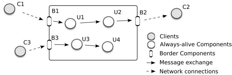
Fig. 1. The ContextChat application.
