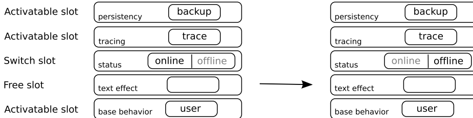
Fig. 9. The context ADT in CONTEXTERLANG. Switching from the online to the offline variation.
